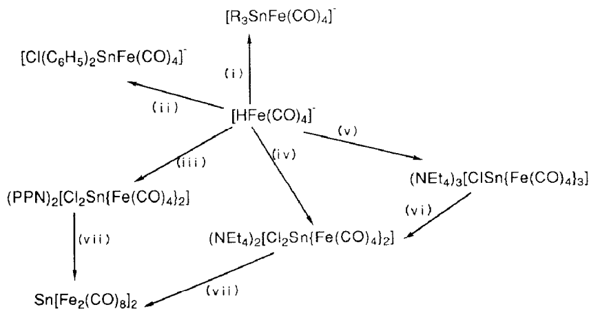
Scheme 1. Reactions of [\text{HFe}(\text{CO})_4]^- with tin compounds. (i) \text{R}_3\text{SnCl} ( \text{R} = \text{C}_6\text{H}_5 , p\text{-C}_6\text{H}_4(\text{CH}_3) ); (ii) \text{R} = \text{Cl}_2\text{Sn}(\text{C}_6\text{H}_5)_2 ; (iii) \text{R} = \text{SnCl}_4 ; (iv) \text{R} = \text{SnCl}_4 (molar ratio 2Fe/1Sn); (v) \text{R} = \text{SnCl}_4 (molar ratio 3Fe/1Sn); (vi) \text{R} = \text{SnCl}_4 ; (vii) \text{R} = \text{Cu}^+ (molar ratio 1Sn/2Cu).
