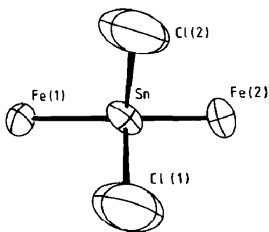
Fig. 1. Skeleton of the anion [\text{Cl}_2\text{Sn}\{\text{Fe}(\text{CO})_4\}_2]^{2-} . Selected dimensions are as follows: \text{Sn}-\text{Fe}(1) 2.58(3), \text{Sn}-\text{Fe}(2) 2.57(3), \text{Sn}-\text{Cl}(1) 2.35(5), \text{Sn}-\text{Cl}(2) 2.35(4) Å; \text{Fe}(1)-\text{Sn}-\text{Fe}(2) 126(1), \text{Fe}(1)-\text{Sn}-\text{Cl}(1) 108(1), \text{Fe}(1)-\text{Sn}-\text{Cl}(2) 111(2), \text{Fe}(2)-\text{Sn}-\text{Cl}(1) 110(2), \text{Fe}(2)-\text{Sn}-\text{Cl}(2) 107(2), \text{Cl}(1)-\text{Sn}-\text{Cl}(2) 89(2)°.
