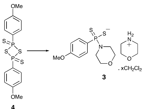
Scheme 1 Synthesis of GYY4137. Conditions: Morpholine (4 equiv.), CH 2 Cl 2 , 0 °C to RT (45–70%). (x = 0.3 to 0.5)
