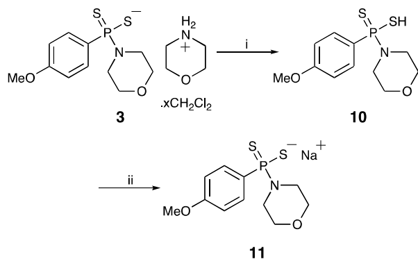
Scheme 4 Synthesis of sodium 4-methoxyphenyl(morpholino)phosphinodithioate 11 . Reagents and Conditions: (i) CH_3CO_2H (12 equiv.), H_2O , 0–5 °C (84%). (ii) NaH (1 equiv.), Et_2O , 0 °C to RT (98%).
