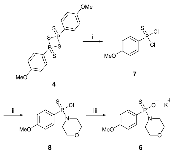
Scheme 3 Preparation of authentic 4-methoxyphenylphosphonamidothioate 6 . Reagents and conditions: (i) SO 2 Cl 2 (3.3 equiv.), CCl 4 , 0 °C, 1 h then RT, 1 h (72% crude), (ii) morpholine (0.9 equiv.), Et 3 N (0.9 equiv.), CH 2 Cl 2 , RT, 1 h (83% based on morpholine), (iii) KOSiMe 3 (2.9 equiv.), Et 2 O, RT, 7 days (94%).
