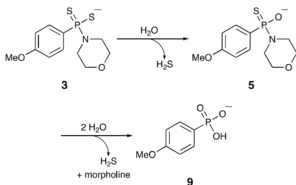
Scheme 2 Two-step hydrolytic degradation of GYY4137 3 . (Note: Counterion for each structure is morpholinium.)
