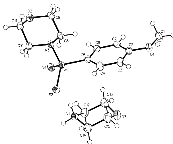
Fig. 2 ORTEP representation of the X-ray crystal structure of GYY4137 3 . Atomic displacement ellipsoids - 50% probability level.
