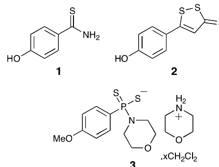
Fig. 1 Slow-release H 2 S donors.
