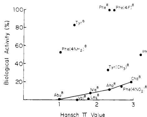
Figure 1. Biological activities of angiotensin II analogues and Hansch \pi values of the substituents in position 8.
