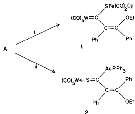
Scheme 2. Reagents. (i) [\text{Fe}(\text{CO})_2\text{CpI}] ; (ii) [\text{AuClPPh}_3] .
