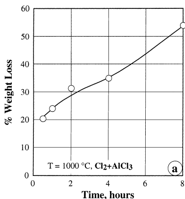
Fig. 5. Evolution of % WL of sample (a) and % Fe and % Cr extraction (b) as a function of time during the chlorination of chromite concentrate using \text{Cl}_2 + \text{AlCl}_3 at 1000^\circ\text{C} .
