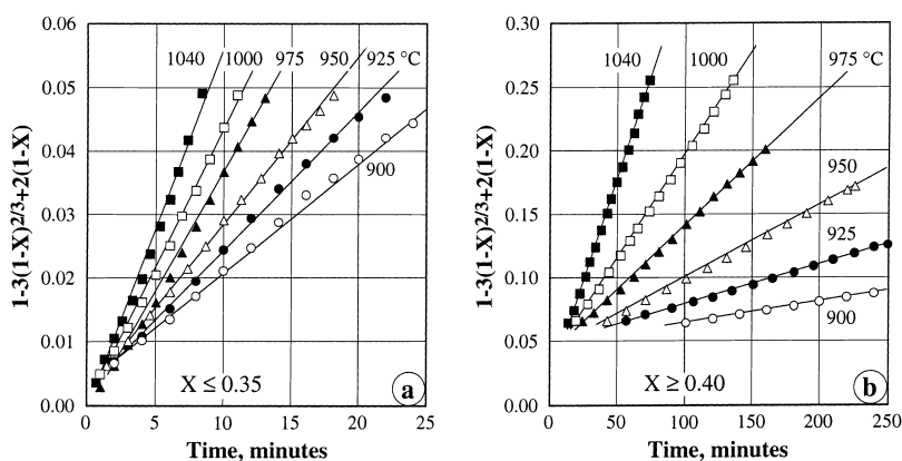
Fig. 8. Mathematical fitting of the chlorination data using Eq. (8) for the reaction extents: (a) X \leq 0.35 and (b) X \geq 0.40 .
