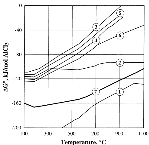
Fig. 4. Evolution of the free-energy changes ( \Delta G^0 ) as a function of temperature for the chlorination with \text{AlCl}_3 of several compounds contained in the chromite [13,14].
