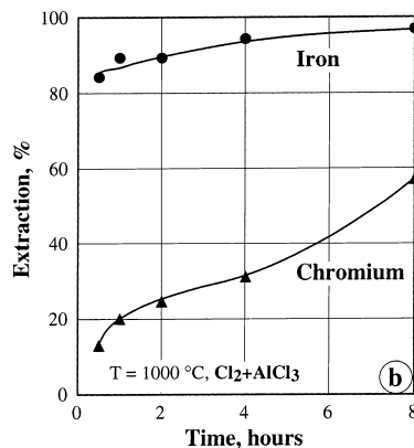
Fig. 5. Evolution of % WL of sample (a) and % Fe and % Cr extraction (b) as a function of time during the chlorination of chromite concentrate using \text{Cl}_2 + \text{AlCl}_3 at 1000^\circ\text{C} .
