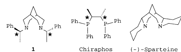
Scheme 4. Chiral chelating ligands.
