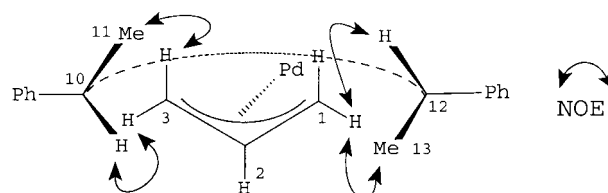
Figure 3. Interligand NOEs observed in [2 \cdot (\text{S,S})\text{-1}] .
