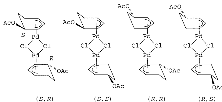
Scheme 1. Species present in a sample of racemic [4-acetoxy-(1,2,3- \eta^3 -cyclohexenyl)palladium ( 4 ).
