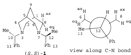
Figure 2. Solution conformation and numbering scheme for 1 .
