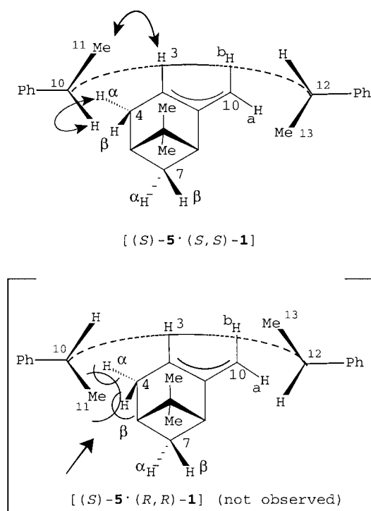
Figure 10. Structurally significant interligand NOEs in the complex formed from ( S )- 5 and ( S,S )- 1 . The structure of the unstable complex formed from ( R,R )- 1 is also shown.
