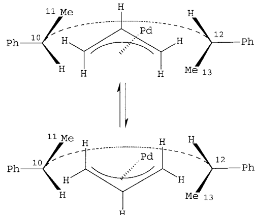
Figure 4. Apparent \pi -allyl rotation in complex [2 \cdot (\text{S,S})\text{-1}] .
