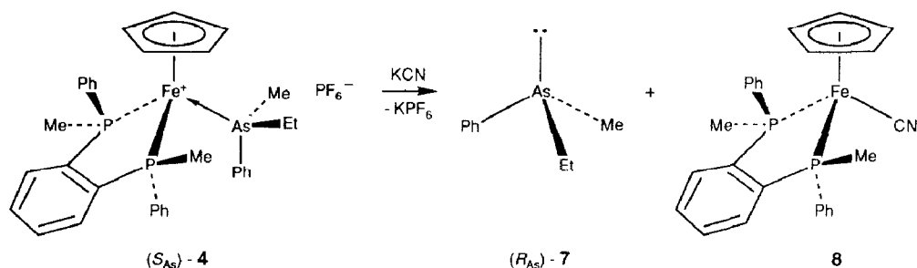
Scheme 4
