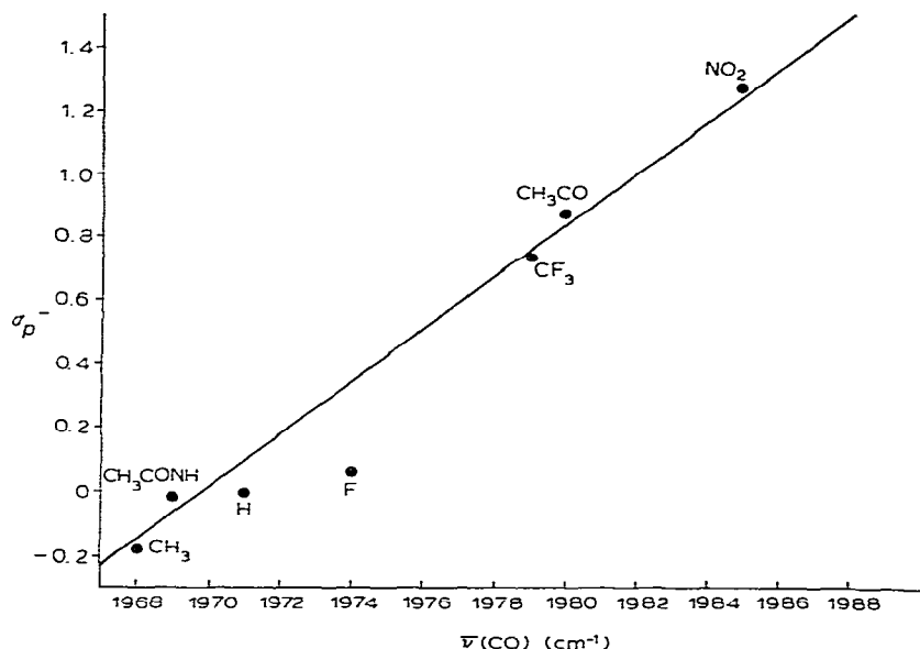
Fig. 1. Correlation between \nu(\text{CO}) and \sigma_p^- for R in \text{Fe}(\text{N}_2\text{C}_6\text{H}_5\text{R})(\text{NO})(\text{CO})(\text{PPh}_3) .
