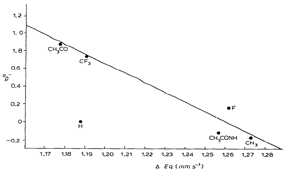
Fig. 2. Correlation between \Delta E_q and \sigma_p^- for R in \text{Fe}(\text{N}_2\text{C}_6\text{H}_4\text{R}-p)(\text{NO})(\text{CO})(\text{PPh}_3) .
