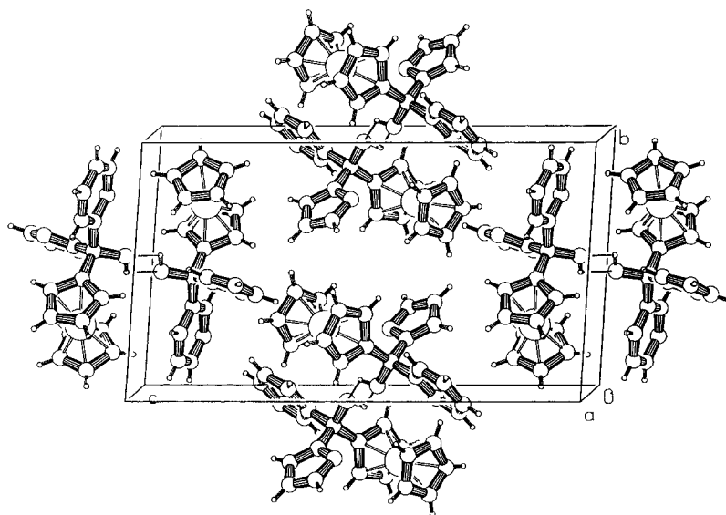
Fig. 3. A view of the crystal structure of 13 .
