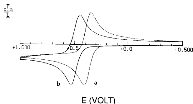
Fig. 4. Cyclic voltammograms recorded at a platinum electrode on \text{CH}_2\text{Cl}_2 solutions containing [\text{NBu}_4][\text{ClO}_4] ( 0.2 \text{ mol dm}^{-3} ) and: (a) 3 ( 1.1 \times 10^{-3} \text{ mol dm}^{-3} ); (b) 20 ( 1.0 \times 10^{-3} \text{ mol dm}^{-3} ). Scan rate 0.2 \text{ V s}^{-1} .
