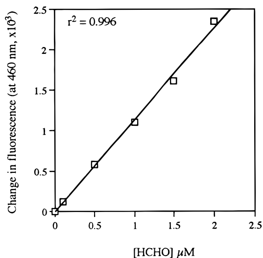
Figure 1. Fluorescence measurements.
