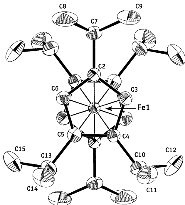
Figure 1. ORTEP diagram of the non-hydrogen atoms of (\text{Cp}^{3i})_2\text{Fe} , giving the numbering scheme used in the text. Thermal ellipsoids are shown at the 30% level.
