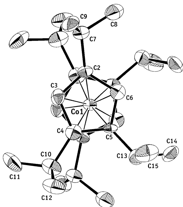
Figure 4. ORTEP diagram of the non-hydrogen atoms of the [(\text{Cp}^{3i})_2\text{Co}]^+ cation ( [\text{BPh}_4]^- salt), giving the numbering scheme used in the text. Thermal ellipsoids are displayed at the 35% level.
