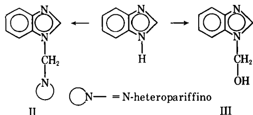
Scheme I—Bachman-Mannich reaction and products.
