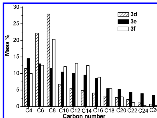
Figure 8. Oligomer distribution obtained in entries 4–6 in Table 2.
