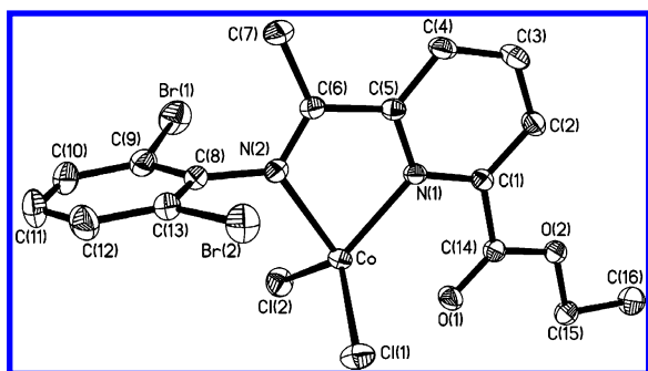
Figure 7. Molecular structure of 4f . Hydrogen atoms and the CH 2 Cl 2 solvate molecule have been omitted for clarity. Selected bond lengths (Å) and angles (deg): Co–N(1) = 2.050(3), Co–N(2) = 2.126(3), Co–Cl(1) = 2.2316(15), Co–Cl(2) = 2.2316(15), Co–O(1) = 2.460; N(1)–Co–N(2) = 77.27(13), N(1)–Co–Cl(2) = 122.43(11), N(2)–Co–Cl(2) = 103.97(10), N(1)–Co–Cl(1) = 116.07(11), N(2)–Co–Cl(1) = 117.20(6), Cl(2)–Co–Cl(1) = 117.20(6).
