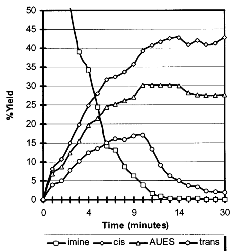
Fig. 1. The reactant and product profile as a function of time. The reaction was performed as usual in \text{CH}_2\text{Cl}_2 at room temperature. The graph illustrates raw data. The % yields are based upon the integration of a peak from each compound against the -\text{CH}_3 peak of the internal standard acetophenone in the ^1\text{H} -NMR spectra of the chronological reaction extracts. The % yields for 3 are not shown due to inconsistencies owing to its volatility during work-up. The curve for the AUEs represents the combined % yields of the three AUE by-products ( 5 , 6 , and 7 ) shown in Eq. (1).
