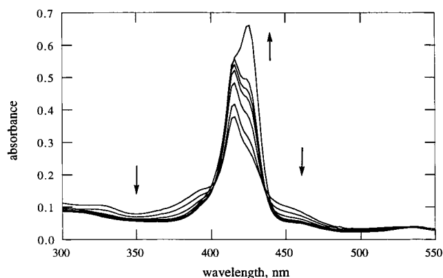
Figure 6. Spectral changes observed with a THF solution of Fe 0 TPP 2- following exposure to 760 Torr of CO 2 . The spectra were recorded at 2, 4, 6, 9, 13, 36, and 150 min after the addition of CO 2 .
