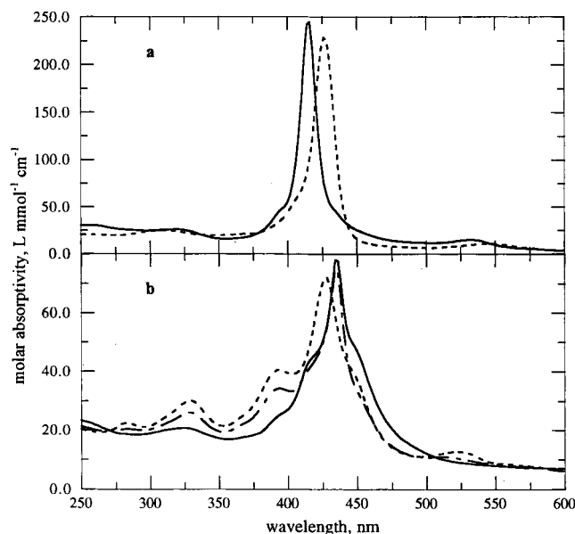
Figure 5. Absorption spectra of Fe II P and Fe I P in THF solutions in the absence and presence of CO. (a) Fe II /T3CF 3 PP (dotted line) and (CO)Fe II /T3CF 3 PP (solid line). (b) Fe I T3CF 3 PP - at room temperature (dotted line), (CO)Fe I T3CF 3 PP - at room temperature (dashed/dotted line), and (CO)Fe I T3CF 3 PP - at low temperature (solid line). The Fe I T3CF 3 PP - solution contains trace amounts of Fe 0 T3CF 3 PP 2- (shoulder at 450 nm) and of (CO)Fe II /T3CF 3 PP (shoulder at 416 nm).
