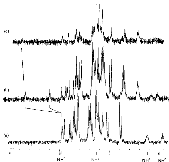
Figure 1. ^1\text{H} NMR spectra of the aromatic/NH region, in \text{CDCl}_3 of: a) Macrocycle 1 ; b) Racemic macrocycle 1 + N -Cbz- \beta -alanyl-L-alanine; c) homochiral macrocycle 1 + N -Cbz- \beta -alanyl-L-alanine
