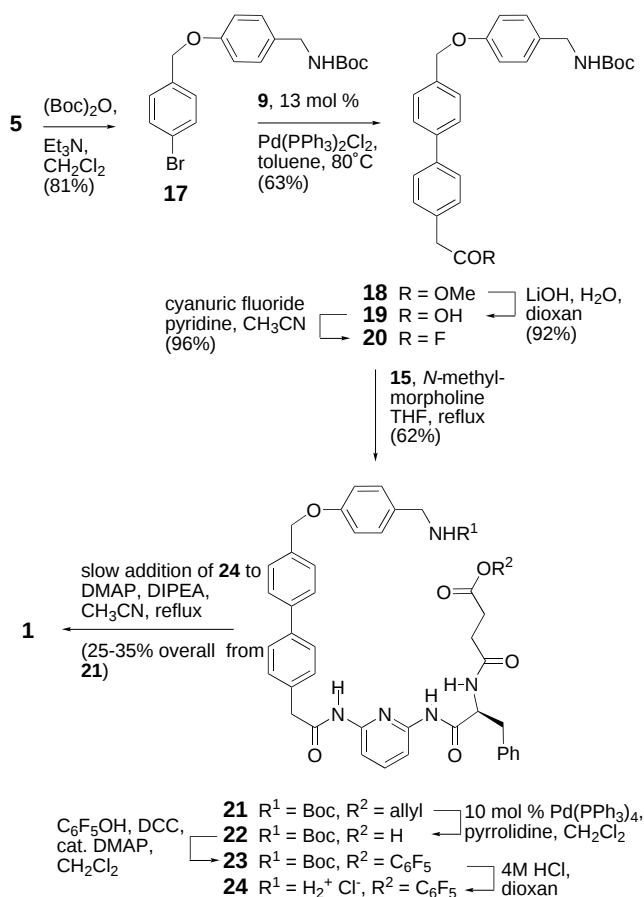
Scheme 3. Synthesis of 1 .
