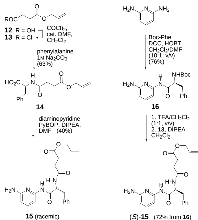
Scheme 2. Synthesis of monoacylated product 15 .
