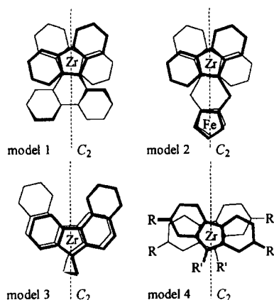
Fig. 2. Four C_2 -symmetric complex models.
