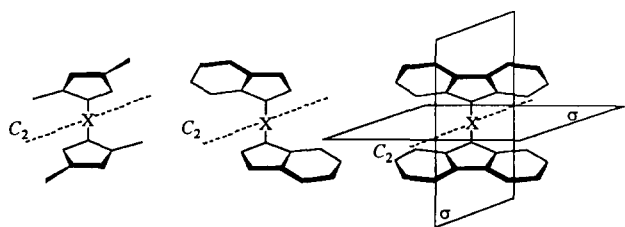
Fig. 1. Comparison of C_2 -symmetric isospecific complexes and highly symmetric aspectic bis(fluorenyl) complexes (schematically).
