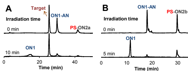
Figure 3. A: HPLC traces (monitored by detecting absorbance at 260 nm) of a mixture of ON1-AN (25 μM), PS-ON2a (1 eq) and Target DNA (1 eq) in annealing solution (pH 7.4, HEPES 6 mM, KOH 5 mM, KCl 20 mM, MgCl 2 0.4 mM) obtained before and after its 10 min-long irradiation with red light (LED array, 650 nm, 0.29 W). B: HPLC traces of a mixture of ON1-AN (20 μM) and PS-ON2b (1 eq) in annealing solution obtained before and after its 5 min-long irradiation with red light.
