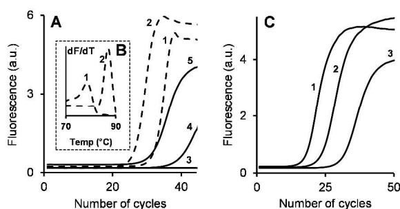
Figure 4. A: Amplification of cDNA derived from \beta -actin-mRNA by using (RT)-PCR; SYBR Green I fluorescence ( \lambda_{em} = 521 nm, \lambda_{ex} = 494 nm) was monitored: (1) ON1 (1 eq), PS-ON2a (1 eq), ON3 (1 eq, C_p = 29); (2) the same as (1) except total RNA (15 ng) was added ( C_p = 25); (3) ON1-AN (1 eq), PS-ON2a (1 eq), ON3 (1 eq), total RNA (150 ng, no amplification detected), the same result was obtained with 15 ng total RNA; (4) the same as (3) except total RNA (15 ng) was added and the mixture was irradiated for 10 min with LED light source (650 nm, 0.29 W) in the annealing buffer ( C_p = 40); (5) the same as (4) except more total RNA (150 ng) was added ( C_p = 31). B: Fluorescence melting profiles (dF/dT versus T) of products obtained in reactions (1) and (2) from A. C: RT-PCR of \beta -actin-cDNA: (1) ON1 (1 eq), PS-ON2b (2 eq), ON3 (1 eq), total RNA (150 ng, C_p = 17); (2) ON1-AN (1 eq), PS-ON2b (2 eq), ON3 (1 eq), total RNA (150 ng) and 10 min irradiation in the annealing buffer before the reverse transcription (RT) ( C_p = 23); (3) the same as (2) except the irradiation was conducted in the master mix ( C_p = 31).
