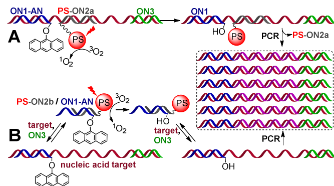
Figure 1. Two designs (A and B) of red-light activated primers for polymerase chain reaction (PCR). PS= photosensitizer, primers: ON1 and ON3, “caged” primer: ON1-AN, amplified nucleic acid: nucleic acid target.
