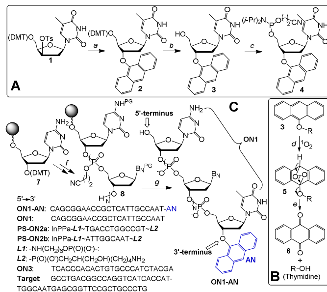
Figure 2. A: Synthesis of phosphoramidite 4 : (a) anthrone, NaH, DMSO; (b) CCl 3 CO 2 H, CH 3 CN; (c) 2-cyanoethyl-N,N-diisopropylchlorophosphoramidite, ( i -Pr) 2 NEt, CH 2 Cl 2 . B: The mechanism of the reaction of 3 with 1 O 2 (steps d-e). C: A list of conjugates described in this paper and an outline of synthesis of ON1-AN: (f) reverse DNA synthesis; (g) 1) 4 , 1H-tetrazole, 2) Ac 2 O, pyridine, N-methylimidazole, 3) I 2 , pyridine, H 2 O, THF, 4) CCl 3 CO 2 H, CH 2 Cl 2 .
