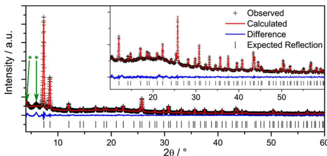
Fig. 2. Pawley fit of UiO-66 obtained from a flow reactor in a two-syringe configuration. Cell refined to a = 20.7367(4) Å (space group: Fm\bar{3}m ; R_{wp} = 5.59\% , \chi^2 = 3.644 ), consistent with reported lattice parameters. 20 Green arrows indicate forbidden reflections.
