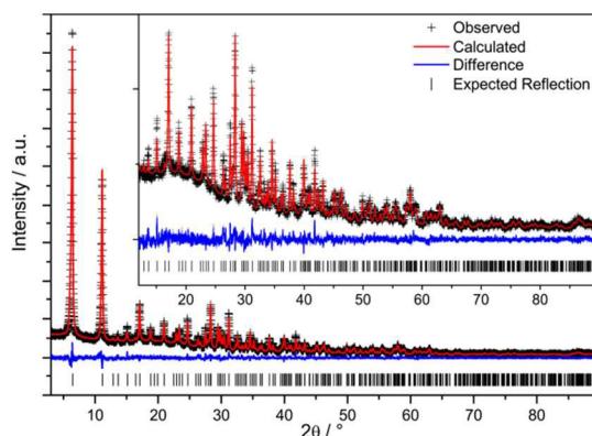
Fig. 6. Rietveld plot of STA-12(Cd) (left) obtained from flow reactor and the structure determined (right). The final cycle of refinement gave R_{wp} = 6.43\% , R_{Bragg} = 1.56\% and \chi^2 = 1.141 .
