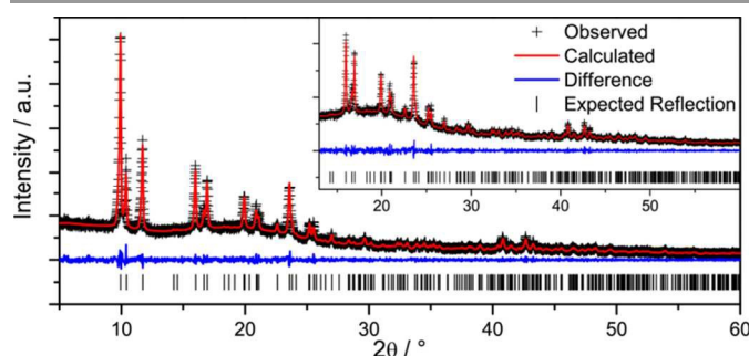
Fig. 3. Pawley fit of CAU-13 obtained from a flow reactor in a two-syringe configuration. Cell refined to a = 6.6111(4) Å, b = 9.4498(6) Å, c = 9.4652(5) Å, \alpha = 107.652(4)^\circ , \beta = 107.690(6)^\circ and \gamma = 93.185(5)^\circ (space group: P\bar{1} ; R_{wp} = 4.71\% , \chi^2 = 1.080 ), consistent with reported lattice parameters. 21
