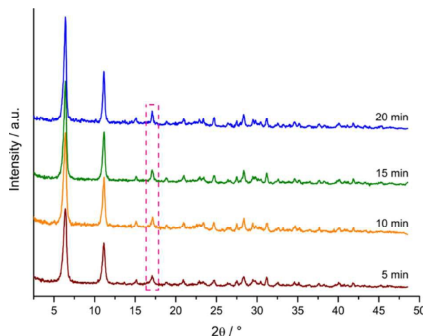
Fig. 5. Samples of STA-12(Cd) prepared in the flow reactor with reaction times increasing from 5 to 20 minutes. Dashed box indicates the (140) reflection, which narrows with increasing reaction time, indicating an increase in particle size.
