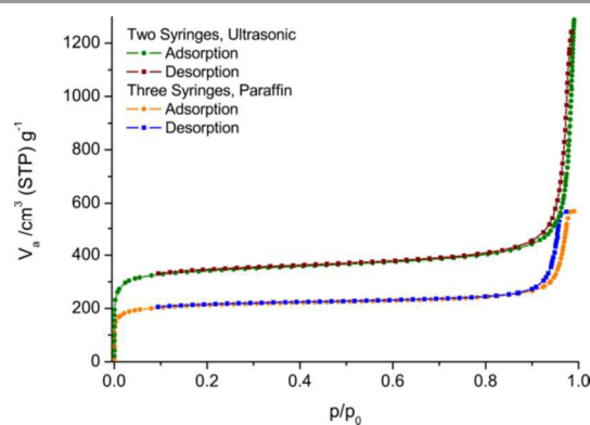
Fig. 3. \text{N}_2 adsorption and desorption isotherms measured at 77 K on samples of UiO-66 produced in a two-pump (ultrasonic probe; green & red traces) and three-pump (paraffin transport; orange & blue traces) flow reactor.
