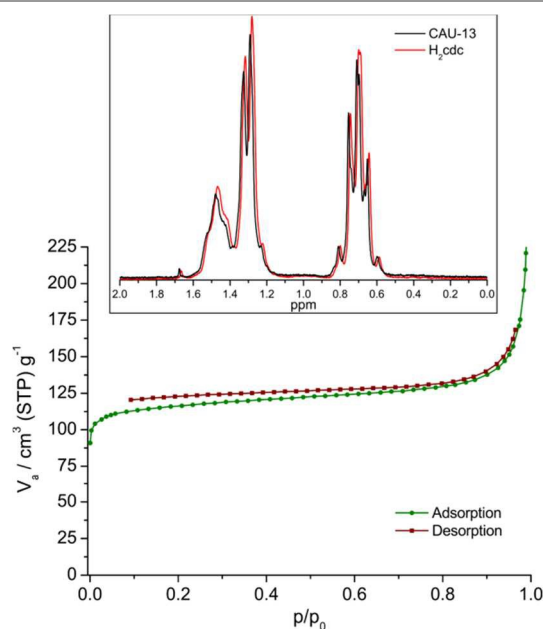
Fig. 4. N_2 adsorption isotherm measured for CAU-13 – a_{BET} = 401 \text{ m}^2 \text{ g}^{-1} . Inset shows the solution state ^1\text{H} NMR spectrum of CAU-13; only resonances attributable to \text{H}_2\text{cdc} were identified and thus no acetic acid was incorporated.
