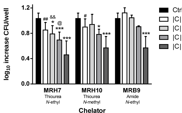
Figure 3. Effect of MRH7 , MRH10 and MRB9 on intramacrophagic growth of M. avium 2447 SmT. BMM were infected with M. avium 2447 SmT. Each chelator was added, just after infection, at a concentration of 5 (a), 10 (b), 20 (c) and 40 (d) \mu M for MRH7 and MRH10 and 15 (a), 30 (b), 60 (c) and 120 (d) \mu M for MRB9 . Infected BMM were incubated for 5 days to measure the intracellular growth of bacteria. The difference, in terms of \log_{10} CFU/well, between days 0 and 5 was designated "log 10 increase". The graphs show the geometric mean \pm SD of the log 10 increase per well obtained from three wells for each condition from three of five independent experiments. Statistical analysis was performed using ANOVA test to compare the bacterial growth: i) in the absence or presence of each the chelators and ii) in the presence MRH7 vs MRH10 vs MRB9 , for the same concentrations, (a), (b), (c) and (d). Statistical significance: * p < 0.05 and ** p < 0.01 when compared with control (no chelator); # p < 0.05 for MRH10 vs MRB9 or ## p < 0.01 for MRH10 vs MRB9 , at concentration (a); * p < 0.05 for MRH7 vs MRB9 , at concentration (b); @ p < 0.05 for MRH7 vs MRB9 , at concentration (c).
