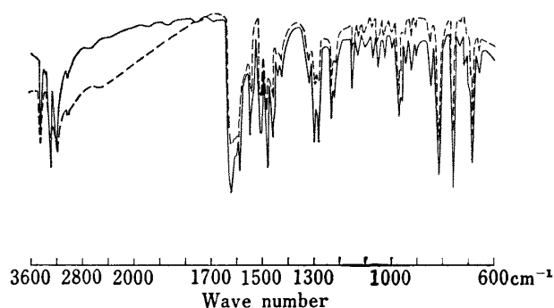
Fig. 6. IR Spectrum of 6-Amino-2-phenylbenzothiazole (KBr)
