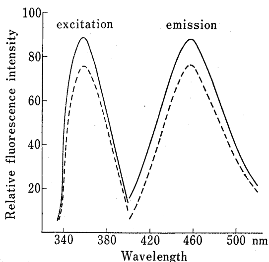
Fig. 1. Excitation and Emission Spectra
