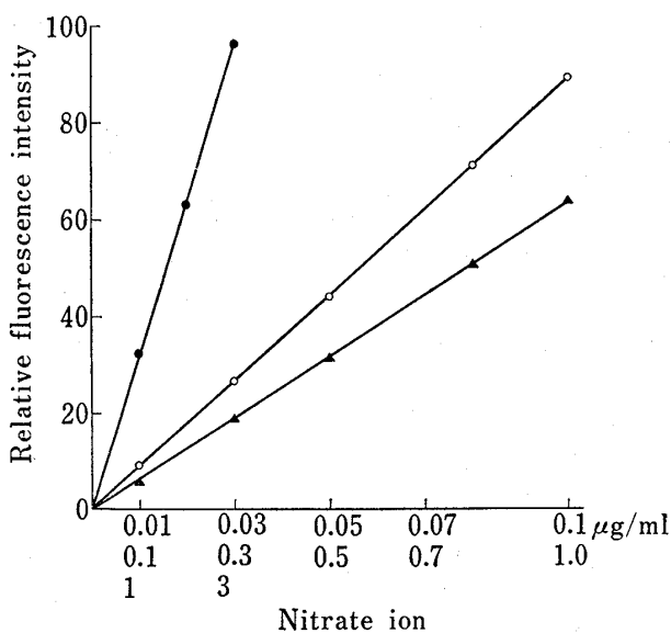
Fig. 2. Calibration Curves for Nitrate
