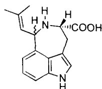
Clavicipitic acid
