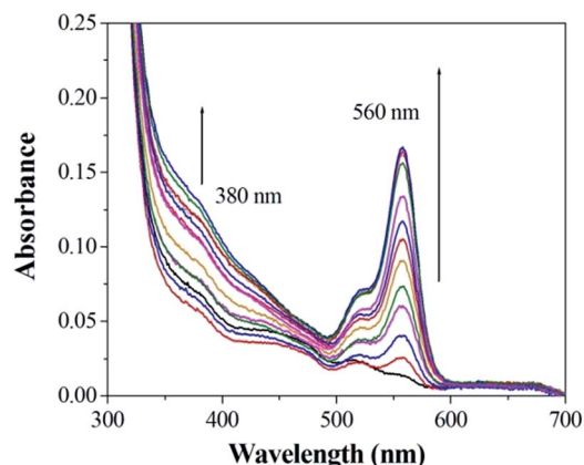
Fig. 6 The absorption change profile of sensor 1 (1 \mu M) to different metal ions (2 mM) in 0.1 M Tris–HCl solution (ethanol–water = 1 : 10, v/v, pH 7.14).
