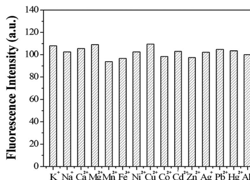
Fig. 9 The fluorescence intensity of sensor 1 ( \mu M) with 1.5 equiv. of \text{Cu}^{2+} , followed by 10 equiv. of \text{M}^{7+} . (Tris–HCl, pH 7.14, ethanol–water = 1 : 10, v/v, \lambda_{\text{ex}} = 500 nm).
