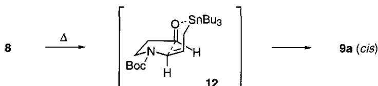
Scheme 2. Cyclic Transition State Model for the Thermal Cyclization of 8
