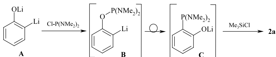
Scheme 3. Proposed mechanism for the formation of compound 2a .
