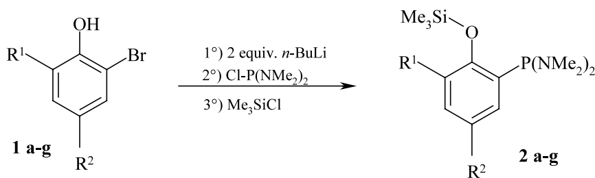
Scheme 2. Synthesis of the key intermediates, o -trimethylsiloxyaryl bis(dimethylamino) phosphines 2 .
