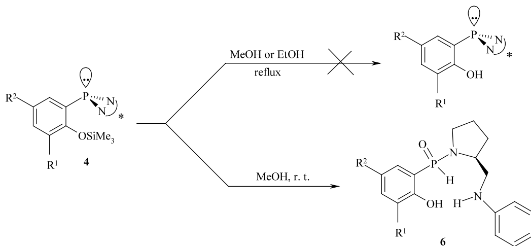
Scheme 5. Methanolysis of the silyl ether function in diazaphospholindines 4 .
