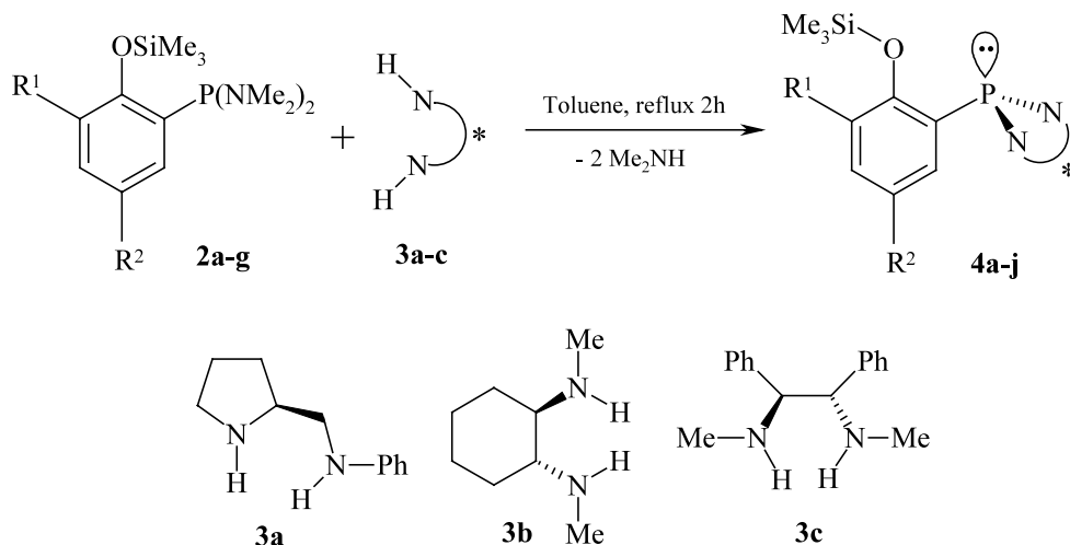
Scheme 4. Synthesis of the o -trimethylsiloxyaryl diazaphospholidines 4 .
