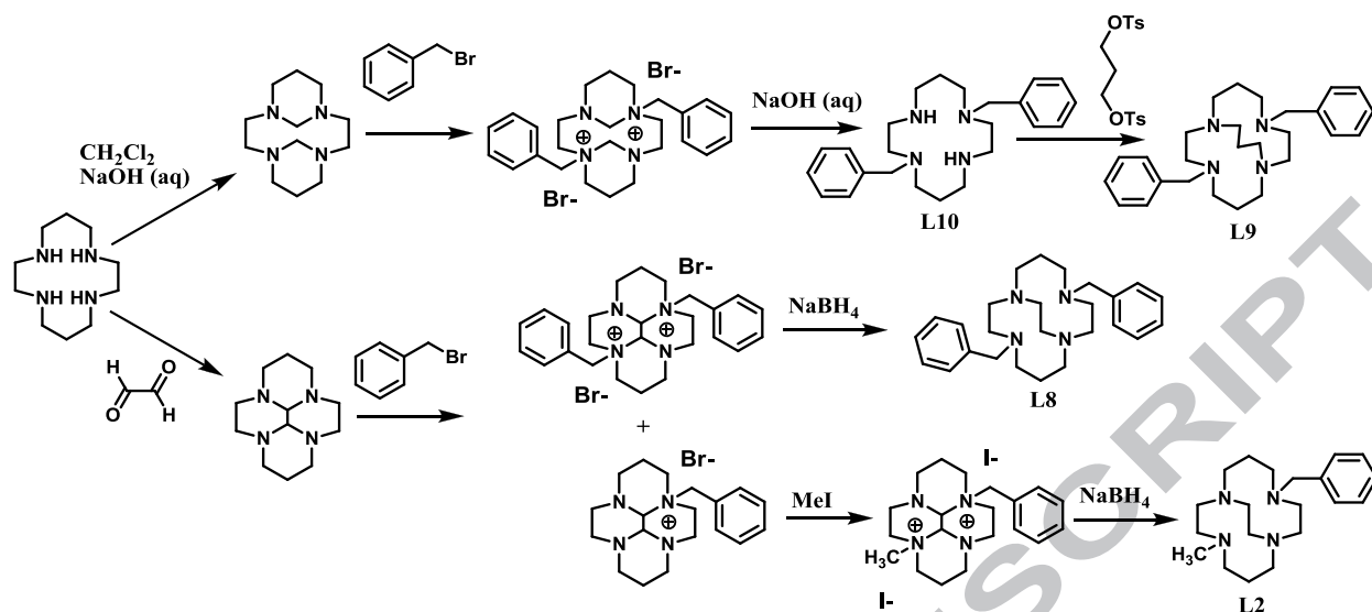
Scheme 1. Synthetic scheme for the literature syntheses of cyclam ligands L2 , 49 L8 , 55 L9 , 54 and L10 . 53 Cyclen analogues L1 , 51 L3 , 55 L4 , 56 and L7 57 are made by analogous reactions.
