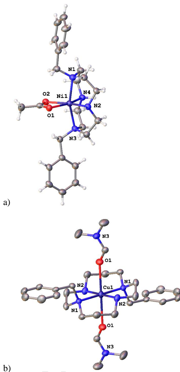
Figure 7. The X-ray crystal structures of a) \text{Ni}(\text{L7})(\text{OAc})^+ (left) and b) \text{Cu}(\text{L10})(\text{DMF})_2^{2+} .
