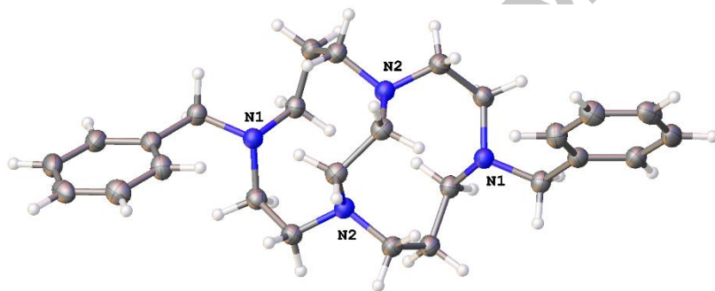
Figure 6. The X-ray crystal structure of L8 .
