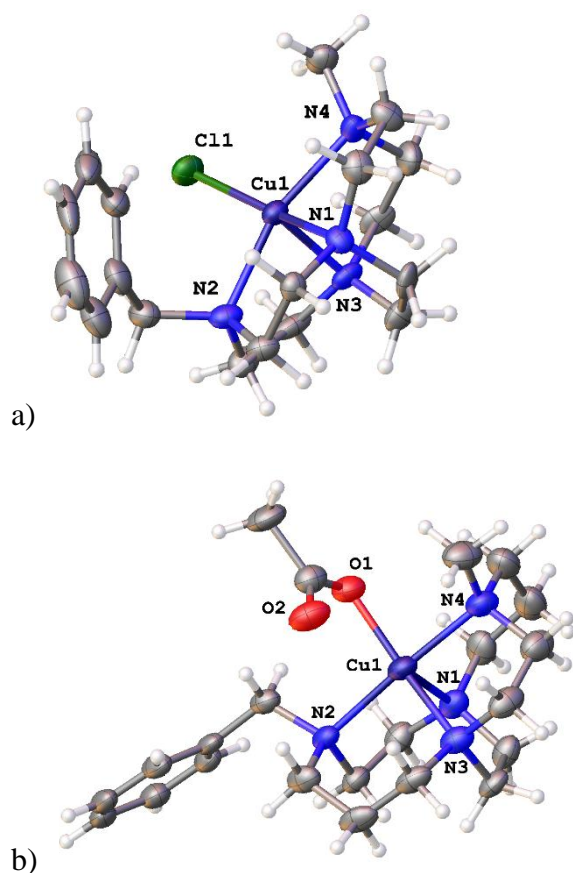
Figure 3. The X-ray crystal structures of a) [Cu(L1)Cl] + (top) and [Cu(L2)(OAc)] + 49 demonstrate the flexibility of the benzyl group, which can fold toward an empty coordination site as in [Cu(L1)Cl] + or away from a more sterically crowded metal ion as in [Cu(L2)(OAc)] + .
