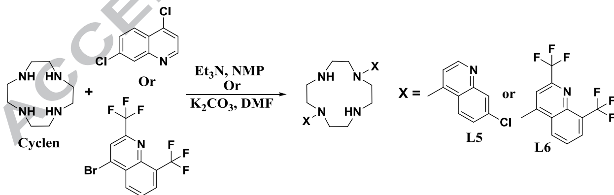
Scheme 2. Synthetic scheme for the literature syntheses of cyclen bisquinoline ligands L5 39,47 and L6 . 47
