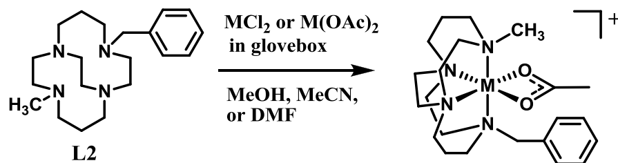
Scheme 3. Generic complexation reaction illustrated using L2 and showing an acetate complex.
