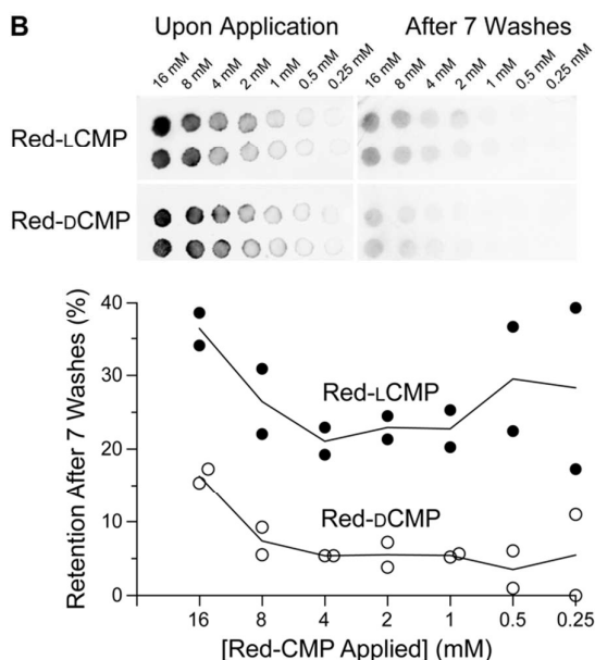
Fig. 4 Images showing the adherence of CMP conjugates and related analytes to collagen surfaces, before and after washing. (A) Photographs of cyanotype paper after being covered by collagen-coated wells that had been treated with Sal-LCMP or a related analyte. (B) Top, Inverse-fluorescence images of Vitro-skin ® spotted with 5 µL of an aqueous solution of Red-LCMP or Red-dCMP (16→0.25 mM). Bottom, Graph of the data as quantified with ImageJ software. 37 For experimental details, see: Supplementary Information, Sections IV–VI.
