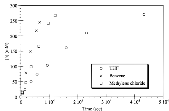
Figure 1. Effect of solvent on the [4 + 1] cycloaddition of 1 with CO.
