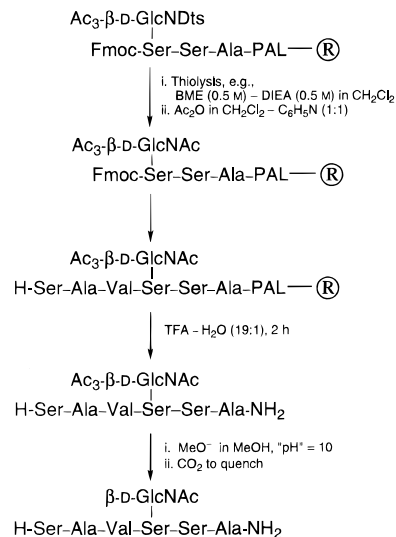
Scheme 4. Solid Phase Synthesis of H-Ser-Ala-Val-Ser(Ac 3 - \beta -D-O-GlcNAc)-Ser-Ala-NH 2 from Dts-Protected Glycosylated Ser and Thr Derivatives
