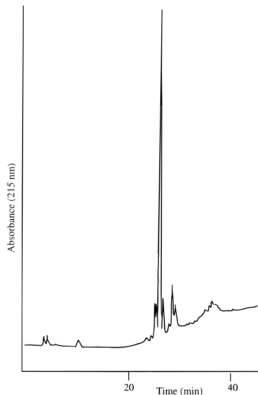
Figure 1. HPLC analysis of H-Ser-Ala-Val-Ser( Ac \beta -D- O -Glc pNAc)-Ser-Ala-NH 2 . HPLC conditions are given in the General Procedures.
