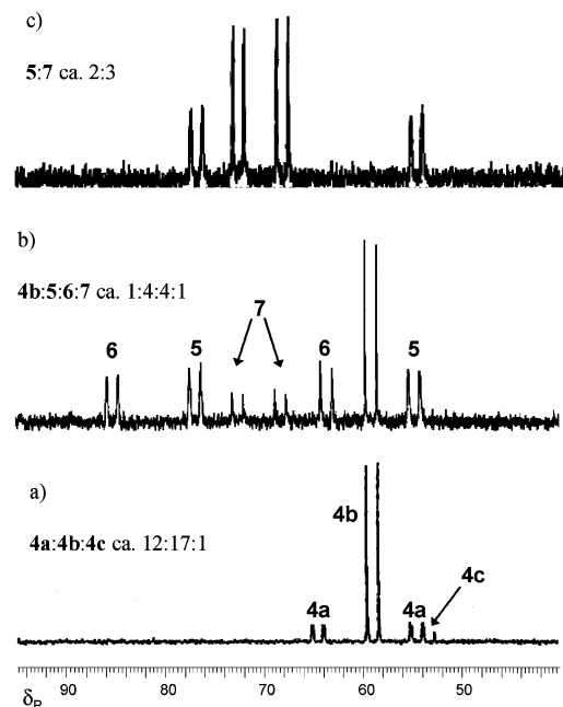
Figure 4. (a) ^{31}\text{P}\{^1\text{H}\} NMR spectrum of 4\cdot\text{BF}_4 in (\text{CD}_3)_2\text{SO} at 25\text{ }^\circ\text{C} : after addition of (b) less than stoichiometric amount and (c) excess of Proton Sponge.
