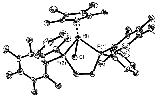
Figure 2. Structure of the SS enantiomer of the cation of [Cp*RhCl( \kappa P, \kappa P- rac -(C 6 F 5 )PhPCH 2 CH 2 PPh(C 6 F 5 ))] [BF 4 ], 4a·BF 4 . Thermal ellipsoids are at the 30% level. Hydrogen atoms are omitted for clarity. Cp*–Rh 1.867(10) Å, Rh–Cl 2.395(2) Å; Rh–P(1) 2.339(3) Å; Rh–P(2) 2.322(3) Å; Cp*–Rh–Cl 120.7(3)°; Cp*–Rh–P(1) 134.2(3)°; Cp*–Rh–P(2) 131.4(3)°; Cl–Rh–P(1) 84.99(9)°; Cl–Rh–P(2) 84.63(9)°; P(1)–Rh–P(2) 84.08(9)°.
