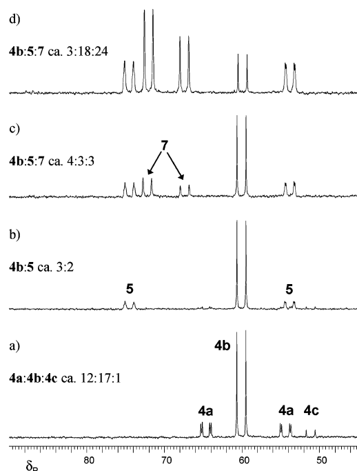
Figure 3. (a) ^{31}\text{P}\{^1\text{H}\} NMR spectrum of 4\cdot\text{BF}_4 in \text{CDCl}_3 at 25\text{ }^\circ\text{C} : (b) 3 h, (c) 66 h, and (d) 238 h after addition of Proton Sponge.
