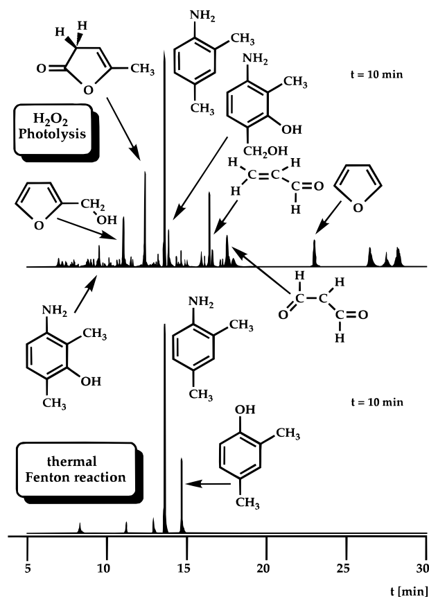
Figure 6. Comparison of the GC/MS traces of 2,4-xylidine and the reaction intermediates formed after 10 min of \text{H}_2\text{O}_2 photolysis and 10 min of the thermal Fenton reaction. (The peak of oxalic acid is not shown due to its interference with the \text{CHCl}_3 peak (solvent for extraction).)
