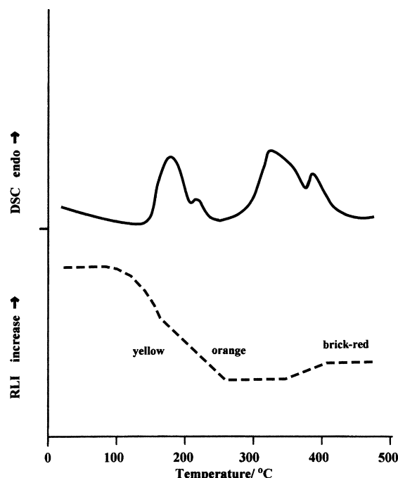
Fig. 2. DSC–RLI of ammonium metavanadate.
