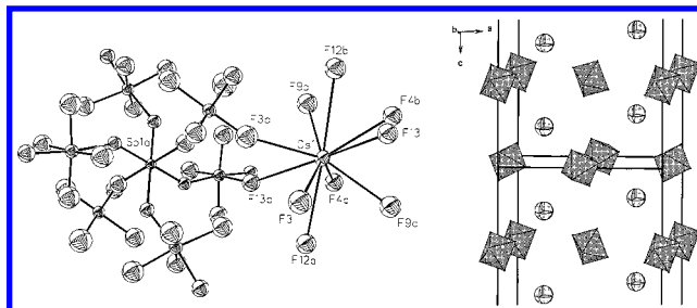
Figure 1. Section of the solid-state structure of \text{Cs}[\text{Sb}(\text{OTeF}_5)_6] ( 1 ). One \text{Sb}(\text{OTeF}_5)_6^- anion and all Cs-F contacts are shown on the left; thermal ellipsoids are drawn at the 25% probability level. The solid-state packing omitting all Te and F atoms is shown on the right ( \text{SbO}_6 octahedra and Cs ellipsoids).
