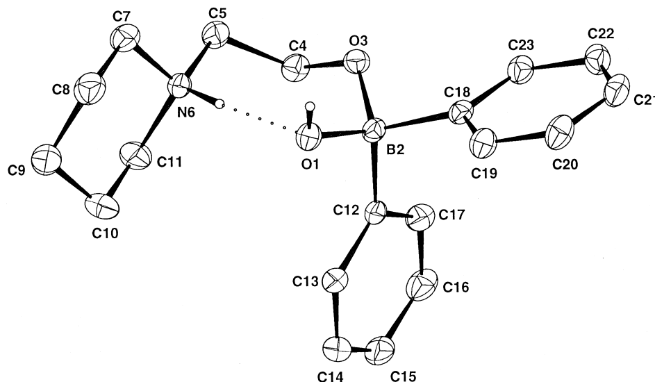
Fig. 1. Molecular structure of compound 12 .
