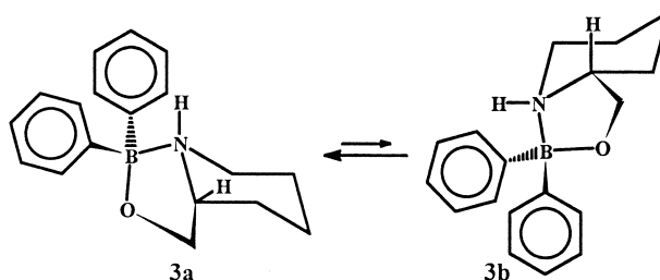
Fig. 4. Conformational equilibrium of compound 3.
