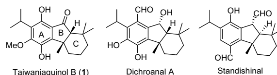
Fig. 1. Representative taiwaniaquinoids.
