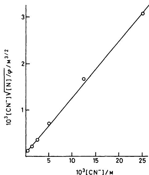
Figure 3. Dependence of the rate of assisted photocyanation of naphthalene (N) on cyanide anion concentration in 1:1 water-acetonitrile. [N] 5 \times 10^{-3} \text{ M} , [DCB] 5 \times 10^{-4} \text{ M}
