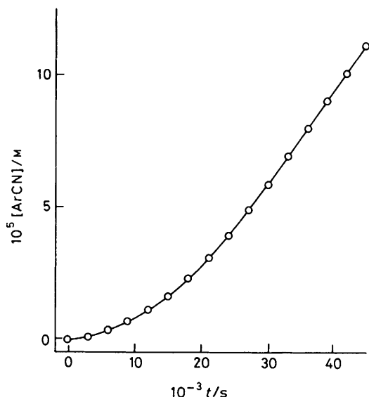
Figure 4. Formation of 9-cyanophenanthrene as a function of irradiation time in autocatalytic photocyanation of phenanthrene (P) in dry acetonitrile. [P] 5.0 \times 10^{-3}\text{M} , [\text{CN}^-] 4.0 \times 10^{-3}\text{M} and [\text{O}_2] 1.2 \times 10^{-3}\text{M}
