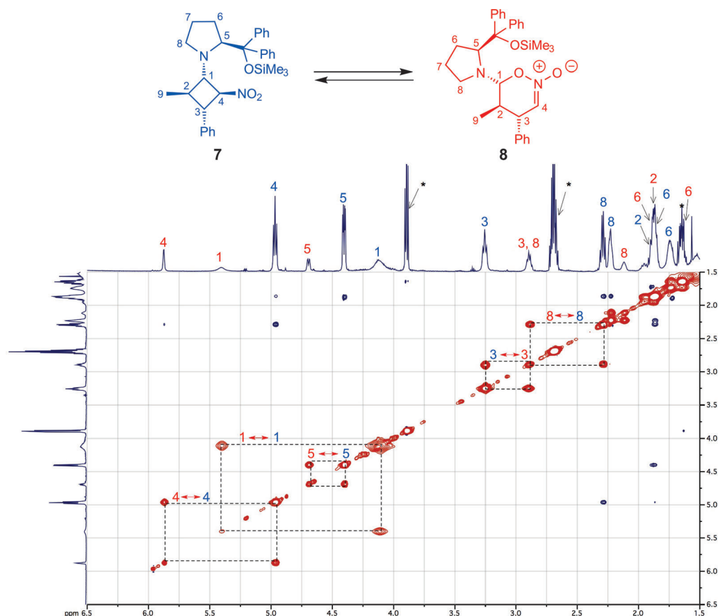
Fig. 3. EXSY Spectrum of the mixture 7/8 ( \text{C}_6\text{D}_6 , r.t., mixing time 500 ms). Immediately after mixing the reactants, the spectrum was recorded which took 1 h to be completed. Peak numbering and colors refer to the H-atoms in positions as shown in the formulae, see also Figs. 1 and 2. For an identical spectrum, see [1r]. The spectrum establishes equilibration between 7 and 8 .
