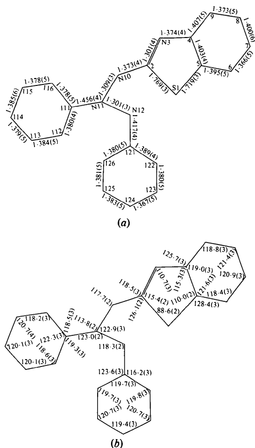
Fig. 2. A schematic drawing of the molecule showing (a) the atom labelling and intramolecular bond lengths (Å) and (b) angles (°), and their associated e.s.d.'s.
