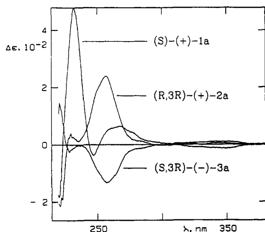
Figure 1. CD spectra of ( S )-(+)- 1a , ( R ,3 R )-(+)- 2a , and ( S ,3 R )-(-)- 3a .
