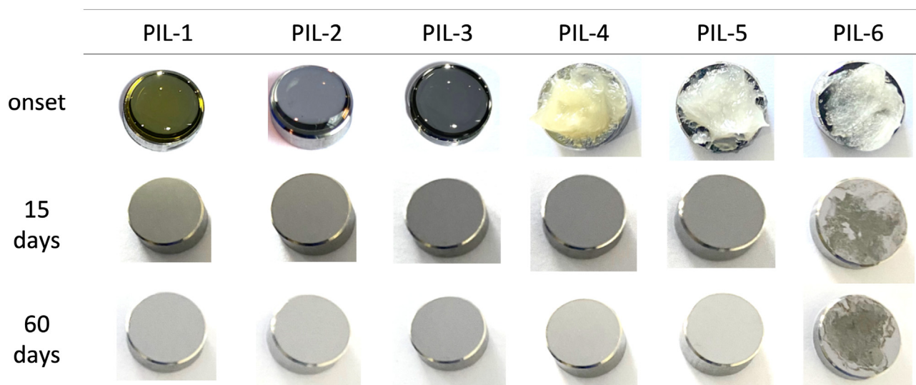
Fig. 4. Disks images during and after corrosion tests.
