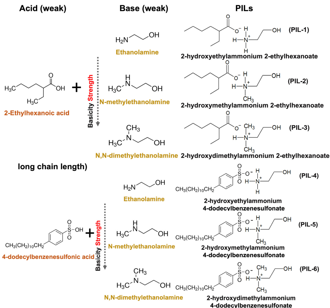
Fig. 1. Simplified procedure of synthesis of each PIL.
