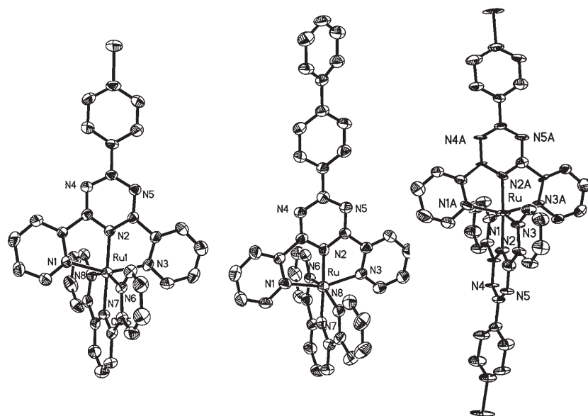
Figure 3. X-ray crystal structure of 2a (left), 2b (center) and 3a (right) as ORTEP representations. Thermal ellipsoids are set at the 50% probability level. The anions and H atoms have been omitted for clarity.
