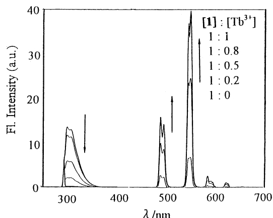
Figure 1. Fluorescence spectra of \text{1} \cdot \text{Tb}^{3+} in \text{CH}_3\text{CN} at 25 °C. [\text{1}] = 1 \times 10^{-5} \text{ M} . Excitation wavelength : 292 nm.
