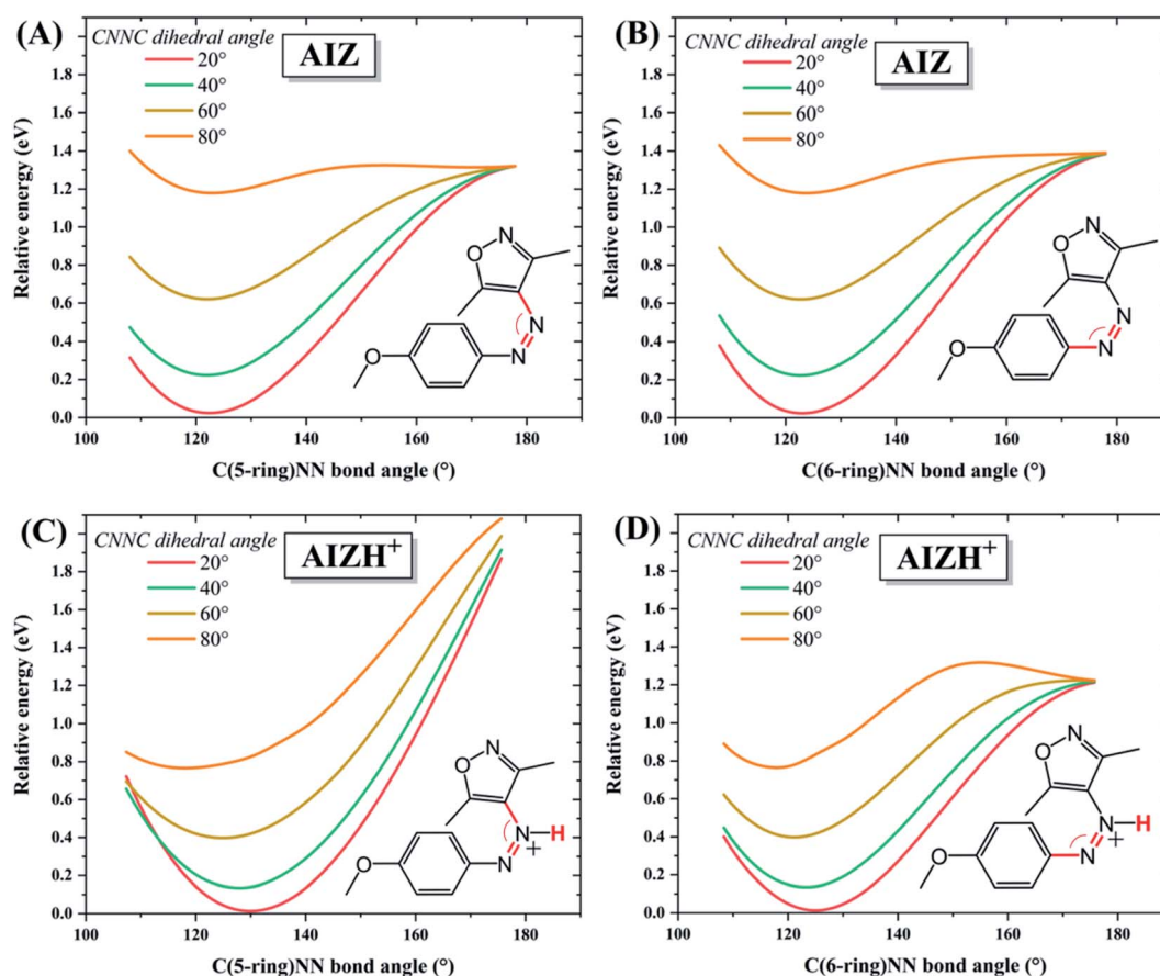
Fig. 3 Relative potential energies of (A and B) AIZ 2 and (C and D) AIZH + 2 along the coordinates of the dihedral angle CNNC (fixed at the values specified), and either (A and C) C(5-ring)NN bond angle or (B and D) C(6-ring)NN bond angle. The amount of data was reduced here for better visualisation, additional data at 10° intervals of CNNC dihedral angle is reported in Fig. S16 † .
