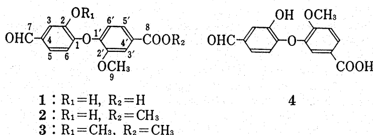
Fig. 2. Possible Structures of Violaceic Acid and Its Methylates
