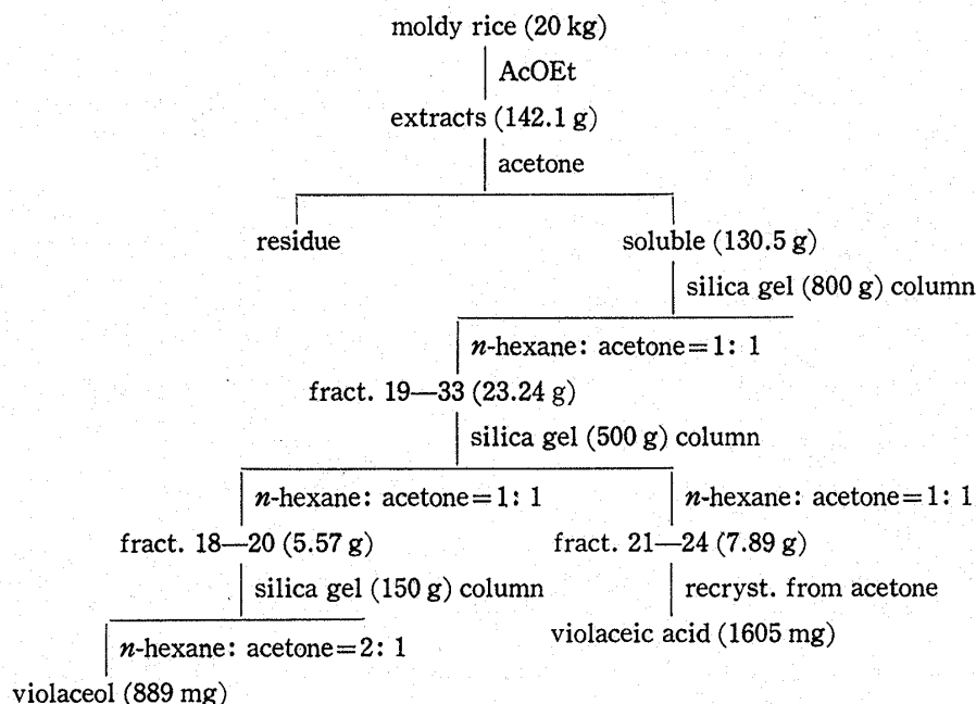
Chart 1. Isolation of Metabolites from Moldy Rice infected with Emericella violacea
