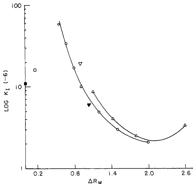
Figure 3. Plot of RDP inhibition vs. lipophilicity: ○, rifazacyclo series; △, rifazone series; ▽, DMB; ▾, DMB analog; ■, rifamazine; □, dirifampin.
