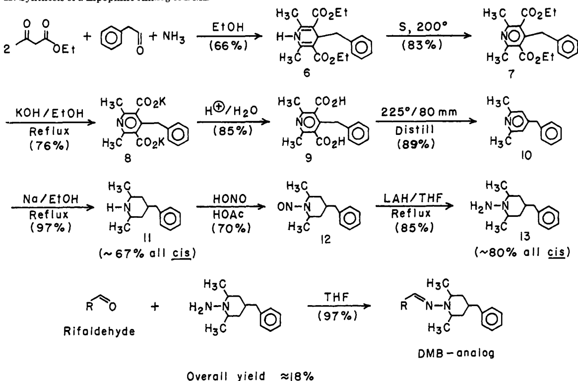
Scheme II. Synthesis of a Lipophilic Analog of DMB
