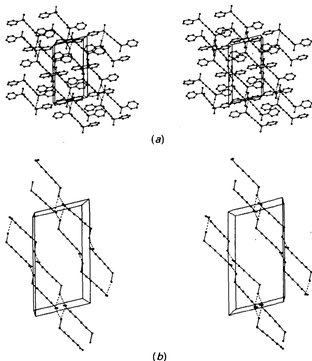
Fig. 3. Stereoscopic view of the crystal packing of rac -(I): (a) only H atoms omitted and (b) methyl and phenyl groups also omitted. Intermolecular O...O proximities suitable for O—H...O hydrogen bonding are indicated by broken lines.
