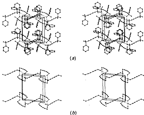
Fig. 2. Stereoscopic view of the crystal packing of meso -(I): (a) only H atoms omitted and (b) methyl and phenyl groups also omitted. Intermolecular O...O proximities suitable for O—H...O hydrogen bonding are indicated by broken lines.
