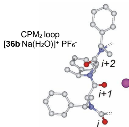
Figure 27. Model of the \text{CPM}_2 loop present in the solid state structure of [\mathbf{36b} \cdot \text{Na}(\text{H}_2\text{O})]^+ \text{PF}_6^- . Hydrogen atoms are omitted for clarity. Atom type: C light grey, N blue, O red, Na magenta.
