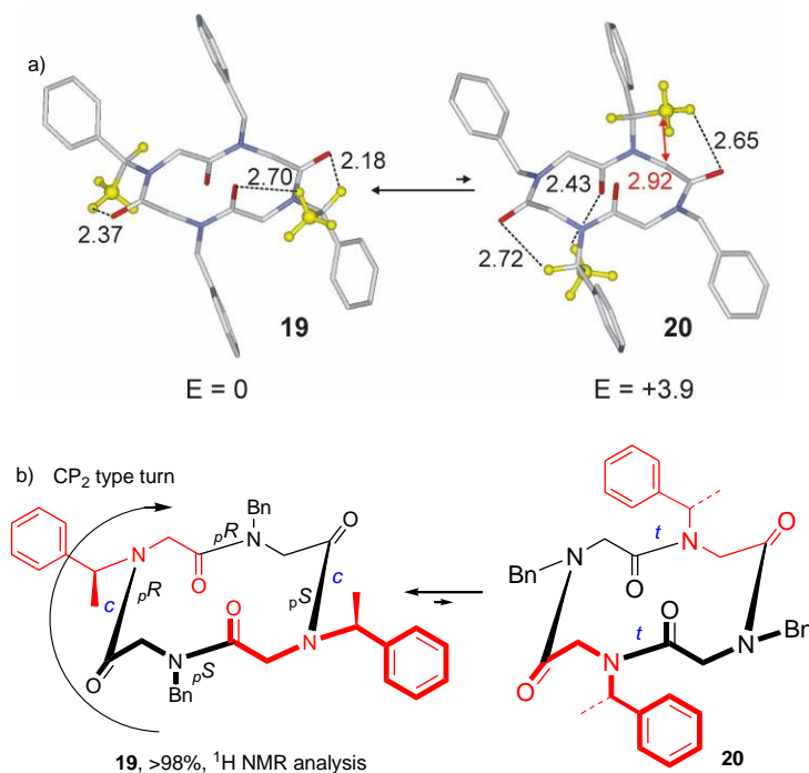
Figure 9. a) Minimum energy structures and their respective internal energies calculated in chloroform and expressed in kcal mol -1 ; distances in black report the favorable hydrogen bonds, in red the unfavorable C-C distance. Hydrogen atoms have been omitted for clarity except some in the Nspe residue (in yellow). Atom type: C light grey (yellow for the CH 3 residues of Nspe ), N blue, O red (see SI for atomic coordinates). Distances are in Å. b) Schematic structures of conformational isomers 19 and 20 with, in red, the chiral residues. The arrow in 19 (following the CO→N direction) depicts CP 2 type β-turn.
