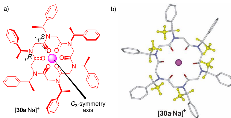
Figure 20. a) Schematic structures of [30a·Na] + with, in red, the chiral residues (Na + as the magenta sphere); b) Minimum energy structure calculated in chloroform. Hydrogen atoms have been omitted for clarity except for the H residues of Nspe (in yellow). Atom type: C light grey (yellow for the CH 3 residues of Nspe), N light blue, O red, Na + magenta (see SI for atomic coordinates).
