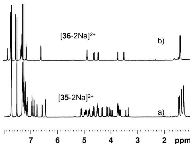
Figure 22. 1 H NMR spectra of a) [35·2Na] 2+ and b) [36·2Na] 2+ complexes as NaTFPB - salts in CDCl 3 (600 MHz, 8.0–1.0 ppm expansion).
