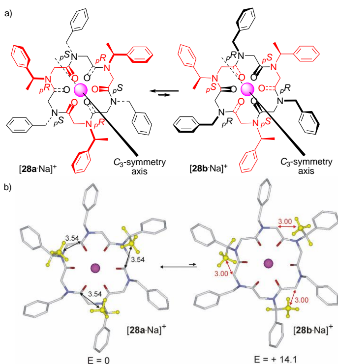
Figure 19. a) Schematic structures of all- trans conformational diastereoisomers [\mathbf{28a}\cdot\text{Na}]^+ / [\mathbf{28b}\cdot\text{Na}]^+ with, in red, the chiral residues (Na + as the magenta sphere); b) Minimum energy structures and their respective internal energies calculated in chloroform and expressed in kcal mol -1 . Hydrogen atoms have been omitted for clarity except for selected H residues of Nspe (in yellow). Atom type: C light grey (yellow for the CH 3 of Nspe), N blue, O red, Na magenta (see SI for atomic coordinates). Distances are in Å.
