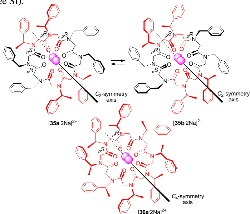
Figure 23. Schematic structures of [\mathbf{35a}\cdot 2\text{Na}]^{2+} , [\mathbf{35b}\cdot 2\text{Na}]^{2+} and [\mathbf{36a}\cdot 2\text{Na}]^{2+} with chiral residues in red ( \text{Na}^+ ions as the magenta sphere).
