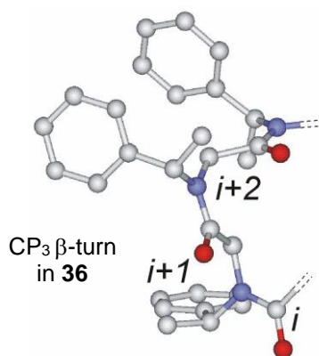
Figure 17. Model of type \text{CP}_3 turn in the minimum energy structures of C_2 -symmetric 36 . Hydrogen atoms are omitted for clarity. Atom type: C light grey, N blue, O red.
