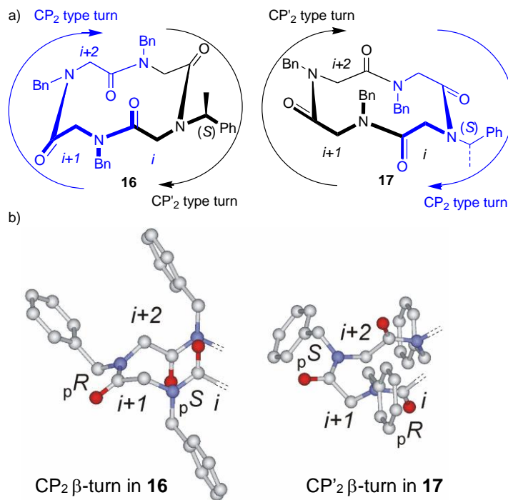
Figure 8. a) Schematic structures of conformational diastereoisomers depicting type CP 2 and CP' 2 β-turns present in 16 and 17 . The arrows point toward the CO→N direction. b) Models of CP 2 and CP' 2 β-turns extracted from the minimum energy structures of 16 and 17 , respectively. Hydrogen atoms are omitted for clarity. Residue i and i +3 are partially omitted for clarity. Atom type: C light grey, N blue, O red.
