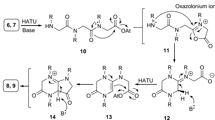
Scheme 1. Suggested mechanism for the formation of pyrrolopyrazine 8 and 9 from high dilution condensation of H- Npm - Nspe 2 -OH ( 6 ) and H- Nspe 3 -OH ( 7 ). At = 7-azabenzotriazole; R = benzyl or ( S )- N -(1-phenylethyl) side chain.
