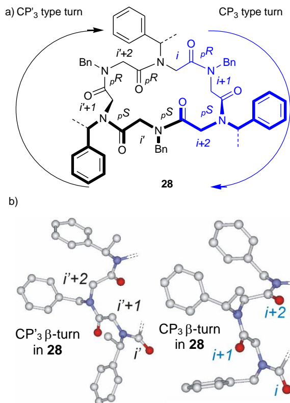
Figure 13. a) Schematic structures of 28 depicting type CP'_3 (in black) and CP_3 (in blue) cct \beta -turns with arrows pointing towards the CO \rightarrow N direction. b) Models of type CP'_3 (left) and CP_3 (right) cct turns present in the minimum energy structures of 28 . Hydrogen atoms are omitted for clarity. Atom type: C light grey, N blue, O red.
