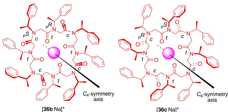
Figure 25. Schematic structures of [36b·Na] + PF 6 - and [36c·Na] + PF 6 - conformational isomers (Na + ion is the magenta sphere).
