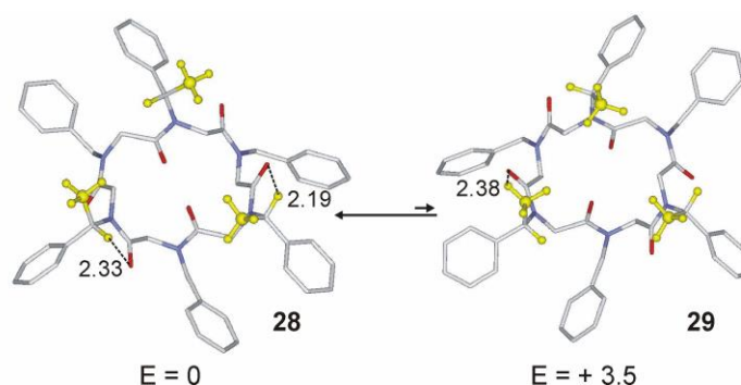
Figure 12. Minimum energy structures of 28 and 29 and their respective internal energies calculated in chloroform and expressed in kcal mol -1 with reported hydrogen bonds as dotted lines (and atomic distances). Hydrogen atoms have been omitted for clarity except some in the Nspe residue (in yellow). Atom type: C light grey (yellow for the CH 3 residues of Nspe ), N light blue, O red (see SI for atomic coordinates). Distances are in Å.
