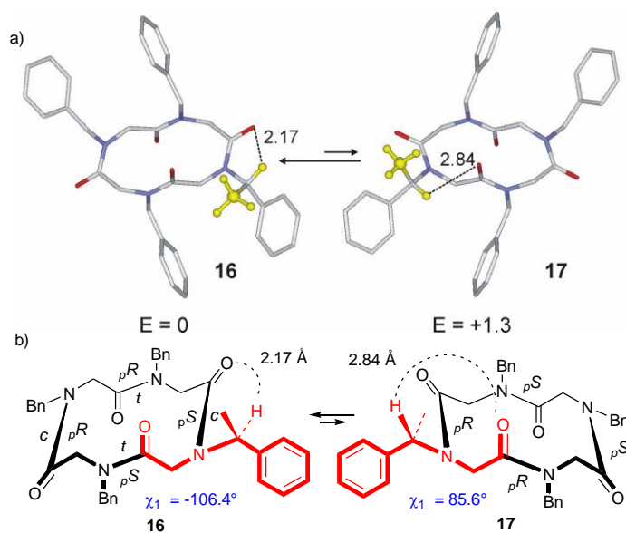
Figure 6. a) Minimum energy and schematic structures of conformational diastereoisomers 16 and 17 and their respective internal energies calculated in chloroform and expressed in kcal mol -1 . Hydrogen atoms have been omitted for clarity except for the CHCH 3 of the Nspe residue (in yellow). Atom type: C light grey (yellow for the CH 3 residues of Nspe ), N blue, O red (see SI for atomic coordinates). Distances are in Å. b) Schematic structures of conformational diastereoisomers 16 and 17 with, in red, the Nspe residue; c = cis ; t = trans .
