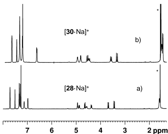
Figure 18. 1 H NMR spectra of a) [28\cdot Na]^+ and b) [30\cdot Na]^+ complexes as NaTFPB salts in CDCl_3 (600 MHz, 8.0–1.3 ppm expansion). Water impurity denoted with *.
