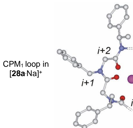
Figure 21. CPM 1 loop present in the minimum energy structures of [28a·Na] + . Hydrogen atoms are omitted for clarity. Atom type: C light grey, N blue, O red, Na magenta.
