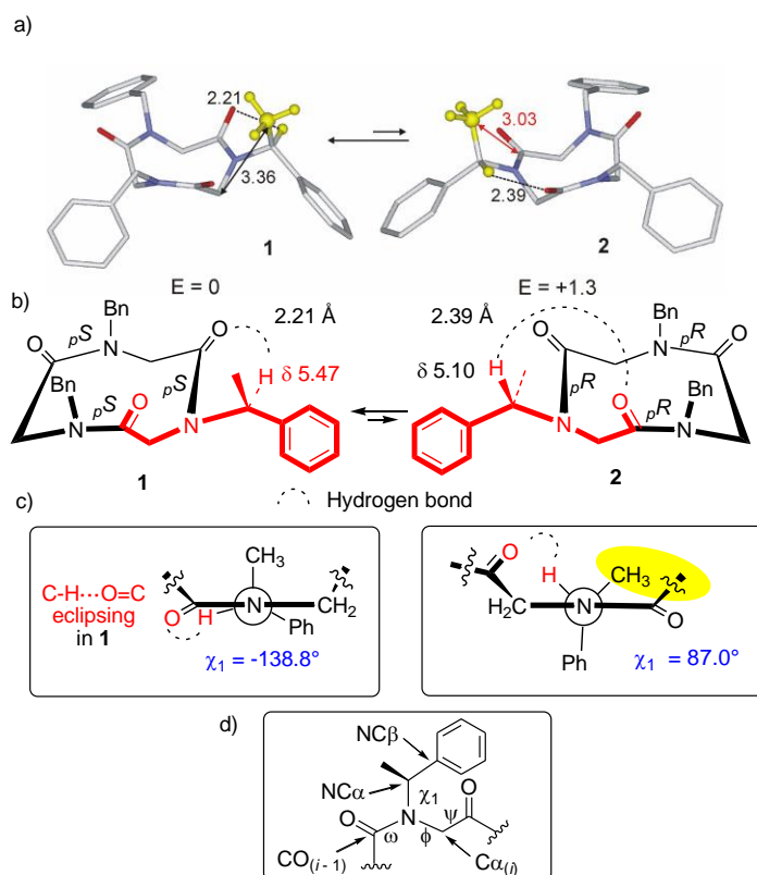
Figure 2. a) Minimum energy structures of 1 and 2 and their respective internal energies calculated in DMSO and expressed in kcal mol -1 (see SI for atomic coordinates). Hydrogen atoms have been omitted for clarity (except for the CH–CH 3 of the N spe residue, in yellow). Atom type: C light grey (yellow for the CH 3 residues of N spe), N blue, O red. Distances are in Å. b) Schematic structures of conformational isomers 1 and 2 , and key hydrogen bond distances. N spe residue is colored in red. c) Newman projections indicating the \chi_1 in conformational isomer 1 and 2 . Evidenced in yellow is the steric clash between methyl and carbonyl group. d) Dihedral angles definition for a hypothetical residue i : 4d,12a,c \omega [ C\alpha_{(i-1)} ; CO_{(i-1)} ; N_{(i)} ; C\alpha_{(i)} ], \phi [ CO_{(i-1)} ; N_{(i)} ; C\alpha_{(i)} ; CO_{(i)} ], \psi [ N_{(i)} ; C\alpha_{(i)} ; CO_{(i)} ; N_{(i+1)} ], \chi_1 [ CO_{(i-1)} ; N_{(i)} ; NC\alpha ; NC\beta ].
