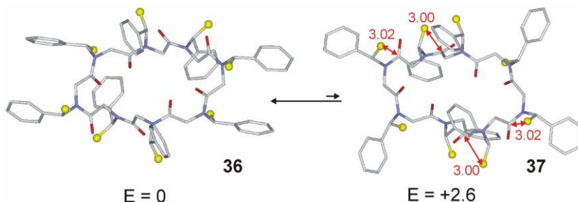
Figure 16. Minimum energy structures of 36 and 37 and their respective internal energies calculated in chloroform and expressed in \text{kcal mol}^{-1} . The unfavorable steric interactions present in conformational isomer 37 evidenced in red. Hydrogen atoms have been omitted for clarity. Atom type: C light grey (yellow for the \text{CH}_3 residues of Nspe ), N light blue, O red (see SI for atomic coordinates). Distances are in Å.
