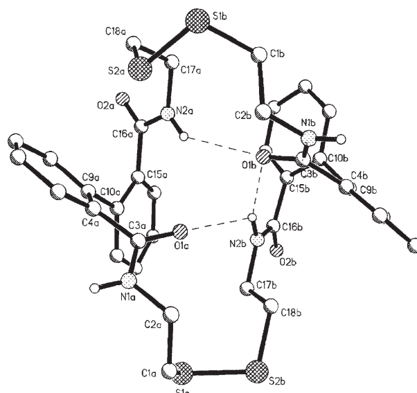
Figure 8. Perpendicular view of 8 .
