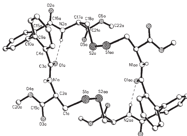
Figure 2. Perpendicular view of 4 . Nine-membered \beta turns are formed with \text{N2a}\cdots\text{O1a} 2.86 Å and \text{H}\cdots\text{O1a} 1.99 Å.
