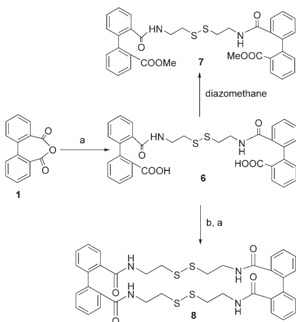
Scheme 2. Preparation of compound 8 . a) cystamine; b) DCC-SuOH.
