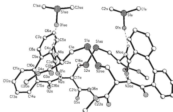
Figure 1. "Edge-on" crystallographic view of 4 . The molecule lies on a true crystallographic two-fold rotation axis. Hydrogen bonds are formed between DMSO molecules and N1a and N1aa, in which \text{N1a}\cdots\text{O1sa} 2.82 Å and \text{H}\cdots\text{O1s} 2.00 Å.
