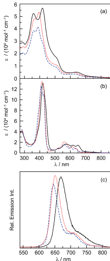
Figure 4. Electronic absorption spectra of the (a) iron XC ( 8a (solid line, black), 8b (dashed line, blue), 8c (dotted line, red)) and (b) the 3H XC ( 4a (solid line, black), 4b (dashed line, blue), 4c (dotted line, red)) series in DCM. (c) Emission spectra of the 3H XC ( 4a (solid line, black), 4b (dashed line, blue), 4c (dotted line, red)) series in DCM.
