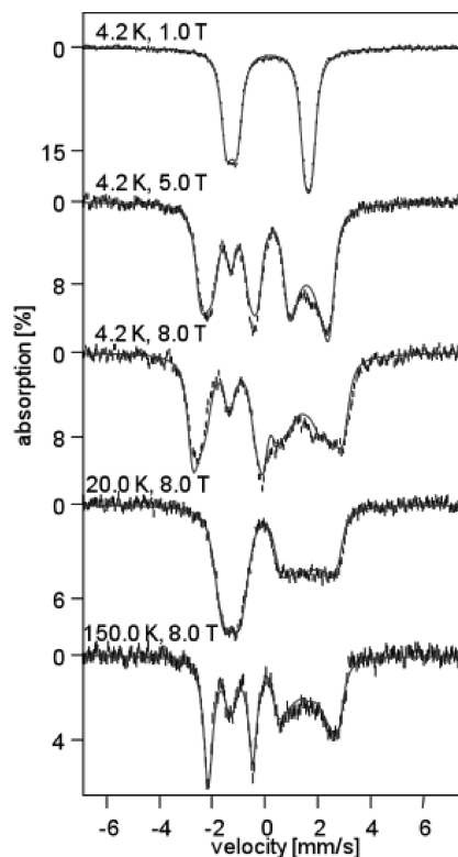
Figure 5. Variable-field, variable-temperature Mössbauer spectra of 8a recorded for a ^{57}\text{Fe} enriched, solid state sample. The applied field is aligned parallel to the incident \gamma beam. The solid lines are best fits obtained using an S = 1 spin Hamiltonian with D = 16.5 \text{ cm}^{-1} , E/D = 0.12 , g_x = g_y = g_z = 2.00 , \delta = 0.193 \text{ mm/s} , \Delta E_Q = 2.911 \text{ mm/s} , \eta = 0.0 , A_x = -24.0 \text{ T} , A_y = -26.7 \text{ T} , A_z = +1.0 \text{ T} and a rotated EFG tensor such that \alpha_{\text{EFG}} = \gamma_{\text{EFG}} = 0.0^\circ , \beta_{\text{EFG}} = 18.0^\circ .
