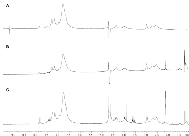
Fig. 1 DF-STD spectra of the 7 -DNA complex. A, B) STD spectra recorded upon saturation in the aromatic (9.0 ppm) and deoxyribose/backbone (2.0 ppm) spectral regions, respectively. C) Reference STD spectrum with an off-resonance irradiation (−16 ppm).
